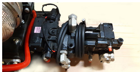
Pump, Drive, Hydrostatic $1,500.00
