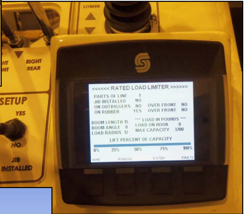
Display panel Information Center with integrated Rated Load Indicator .
